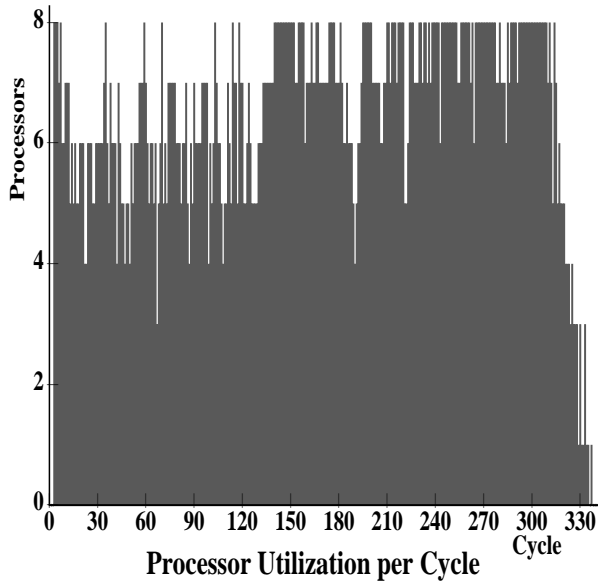
Figure 5: The result of scheduling the 9-body program onto eight Supercomputer Toolkit processors. Comparison with with the region-level parallelism profile (figure 4) illustrates how the scheduler spread the coarse-grain parallelism across the processors. A total of 340 cycles are required to complete the computation. On average, 6.5 of the 8 processors are utilized during each cycle.
